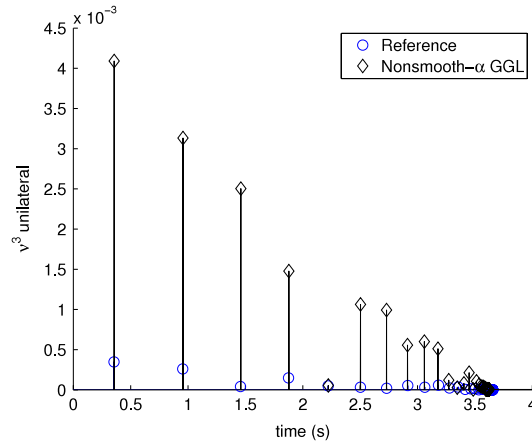
Fig. 11. Bouncing pendulum: unilateral multiplier v^3 .
