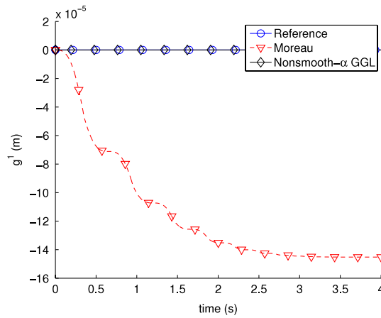
Fig. 12. Bouncing pendulum: bilateral constraint at position level.
