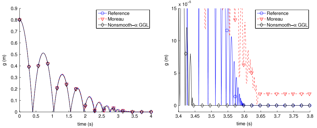
Fig. 4. Bouncing ball: gap distance and zoom.
